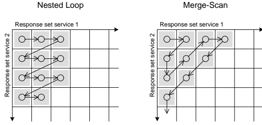
Fig. 9. The Nested Loop and Merge-Scan join strategies.
