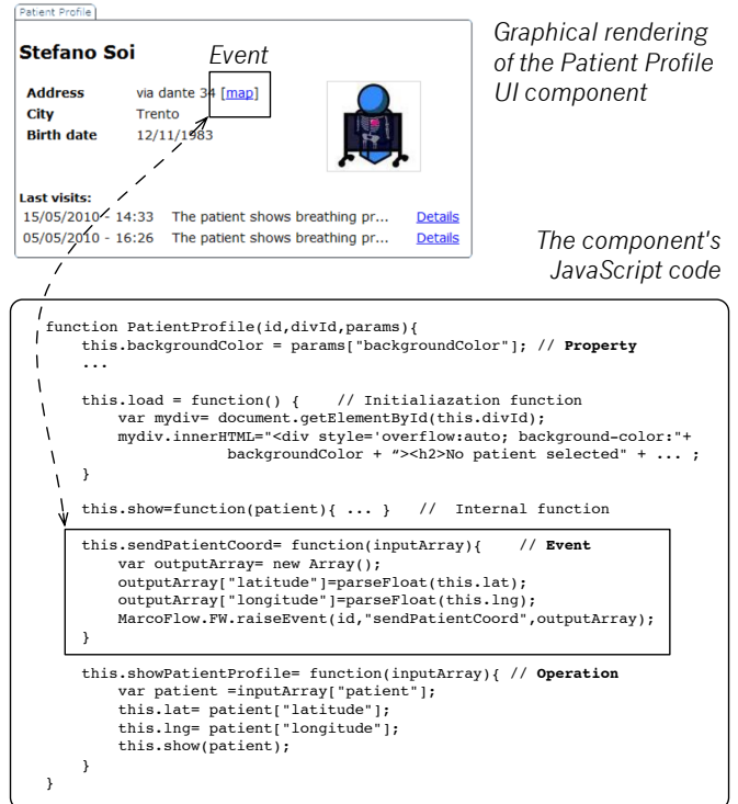
Figure 3: Graphical rendering and internal logic of a UI component
