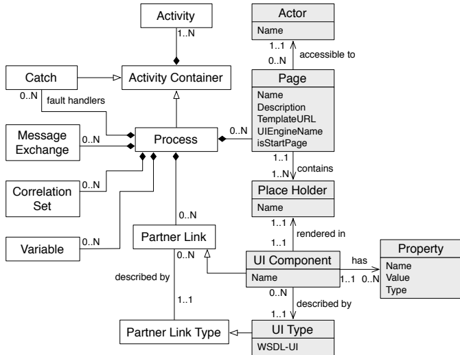
Figure 6: Simplified BPEL4UI meta-model in UML. White classes correspond to standard BPEL constructs [28]; gray classes correspond to constructs for UI and user management.
