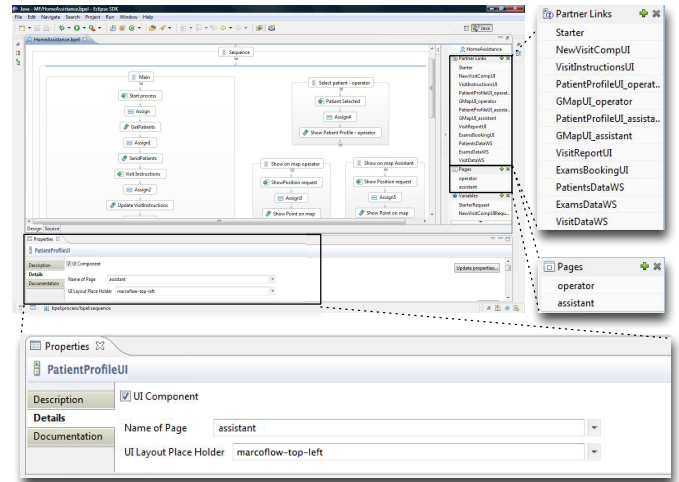
Figure 11: The extended Eclipse BPEL editor for developing UI orchestrations at work.
