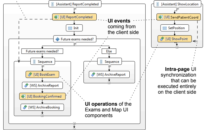
Figure 8: Part of the BPEL4UI model of the home assistance process as modeled in the extended Eclipse BPEL editor (the dashed and dotted lines/arrows have been overlaid as a means to explain the model).
