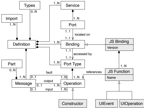
WSDL4UI conventions: (1) All Operations are either UIOperations , UIEvents , or a Constructor . (2) UIOperations only have inputs. (3) UIEvents only have outputs. (4) The Constructor is unique and has only inputs. (5) The service's port address points to the JavaScript class of the UI component.
