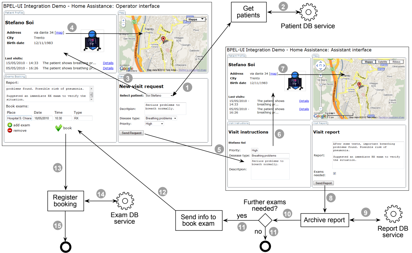
Figure 1: A home assistance application integrating both web services and UI components into a process-like orchestration logic.
