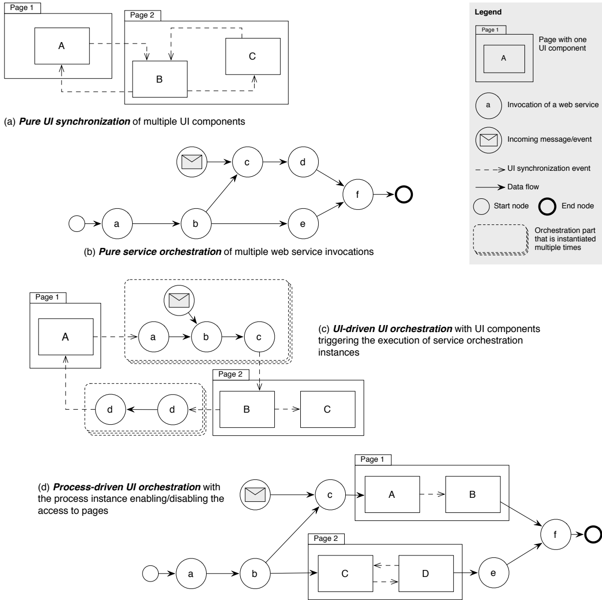
Figure 10: The four types of (UI) orchestration supported by BPEL4UI and the MarcoFlow system.
